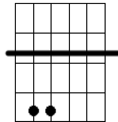
F#m
